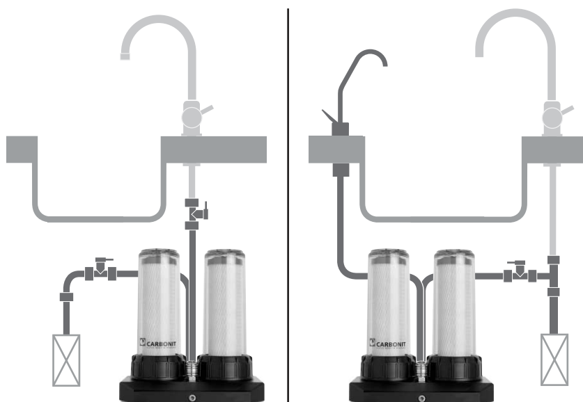
DUO Classic/Clario installation diagram
